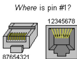
RJ45 Plug and Jack Pin Out
